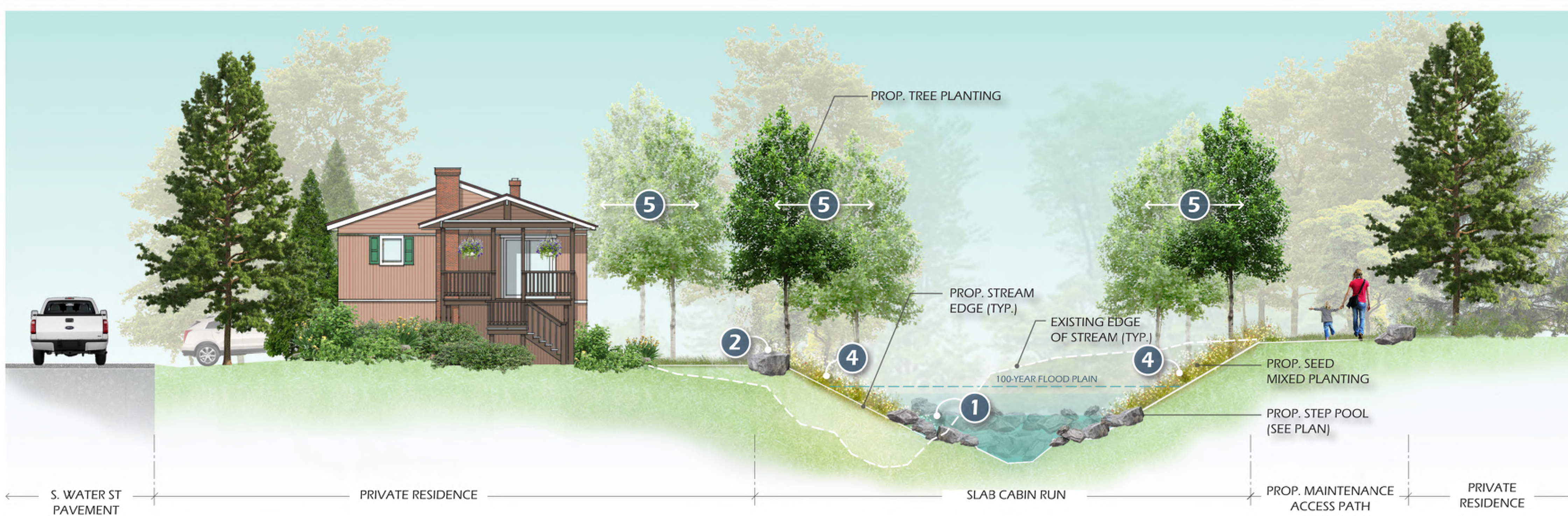
ILLUSTRATIVE SECTION B-B
