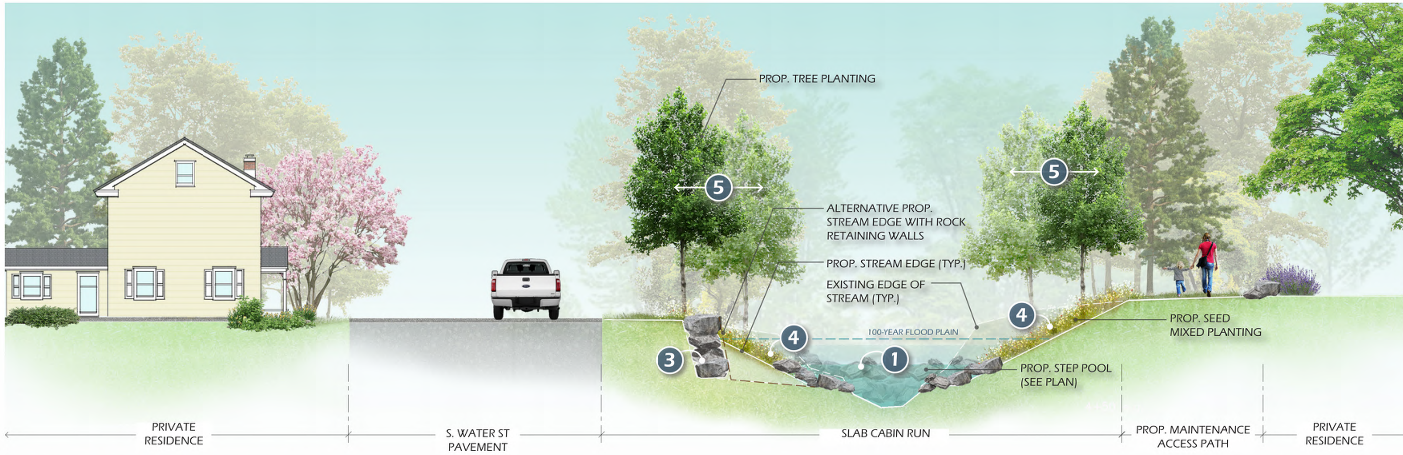
ILLUSTRATIVE SECTION A-A
